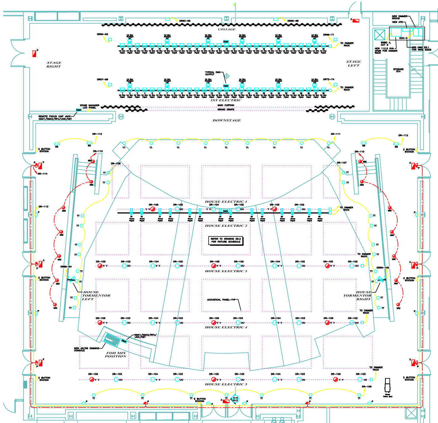
AUDITORIUM THEATRICAL AND HOUSE LIGHTING
